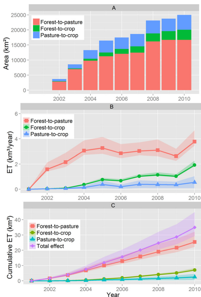
Figure 3. Effect of land use transitions (LUT) on evapotranspiration (ET; from MOD16). (A) Cumulative area of each LUT from 2001–2010. (B) Annual effect of each LUT on ET. (C) Cumulative effect of each LUT on ET. Shaded areas represent the first and third quartiles.
