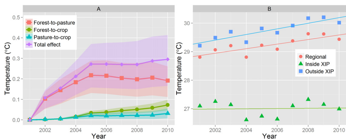
Figure 4. Effect of land use transitions (LUT) on daytime land surface temperature (LST from MOD11A2). (A) Effect on temperature in the entire upper Xingu region during the 2000s for each of three LUTs (shaded areas represent the first and third quartiles). (B) Trends in annual mean surface temperature for the entire upper Xingu basin (regional), inside and outside the Xingu Indigenous Park (XIP).
